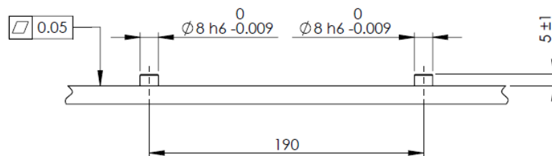
1.2: Monteringsplate for robotbase
